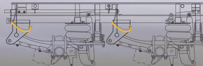
Air/Spring Suspension
