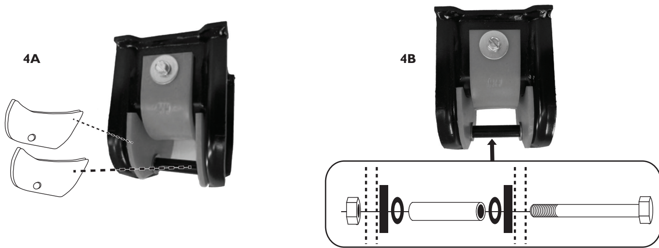
Pictured: A Rear Hanger installed with EWP Warepad and Side Plates.
