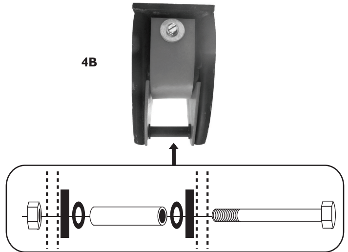
Pictured: A Rear Hanger installed with EWP Warepad and Side Plates.
