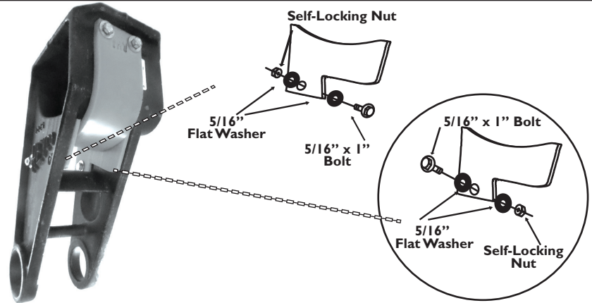
Pictured: A Rear Hanger installed with EWP Warepad and Side Plates.
