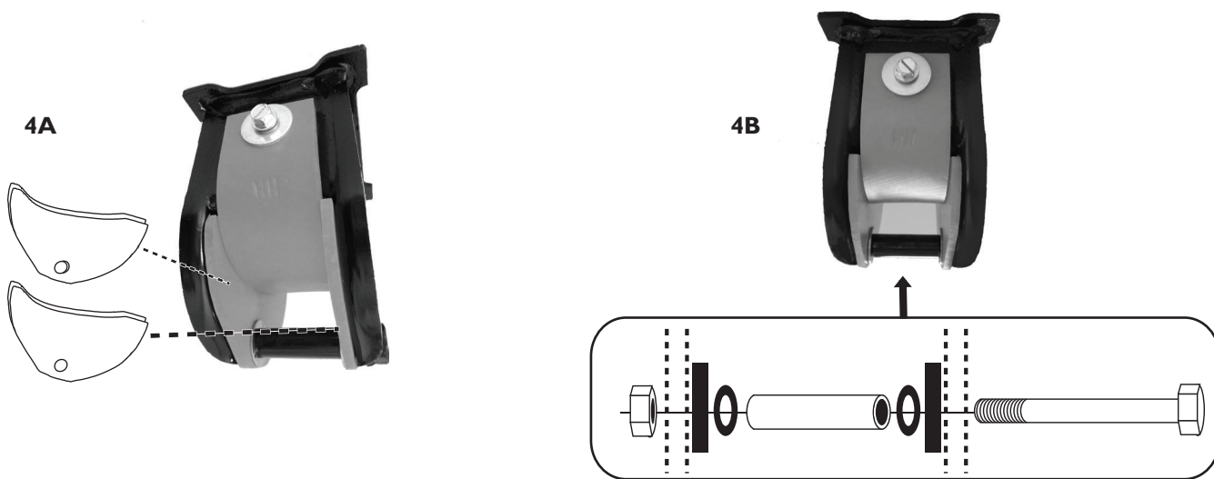
Pictured: A Rear Hanger installed with EWP Warepad and Side Plates.
