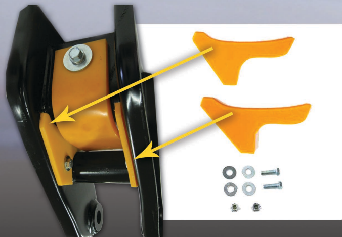
Pictured: Reyco Transpro 88 Fabricated Front Hanger installed with Side Plates & EWP Warepad along with sample of kit which includes Side Plates and fasteners.
